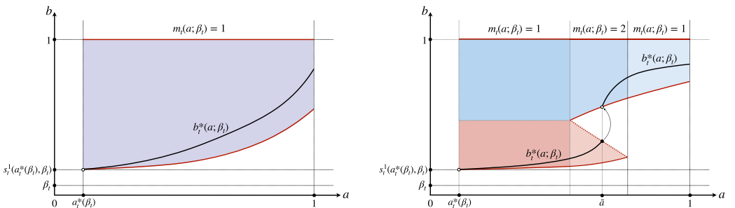
(a) Continuous equilibrium bidding strategy (b) Discontinuous equilibrium bidding strategy
